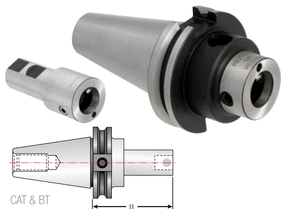
CAT40, CAT50 BT40 Toolholders
