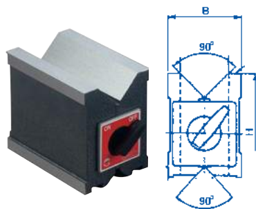
ECE-208 / ECE-212
