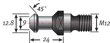
Colombo ISO30 Ball Style for RS Spindles
