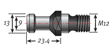
For Colombo ISO30 Billet Spindle
